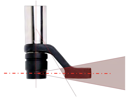
FIGURE 3 – Standard Length Socket Safe Reaction Window
