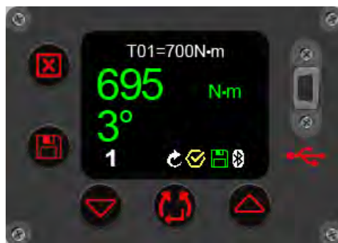
FIGURE 52 – Audit Torque target result (showing achieved torque and output (bolt) movement in degrees)
